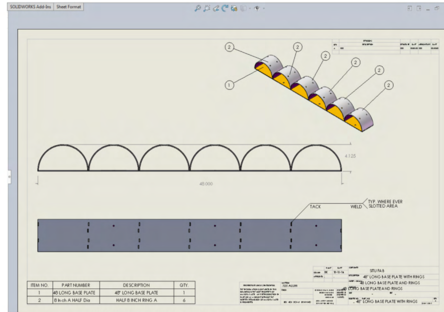
Drawing of base plate & 1 st Row.
